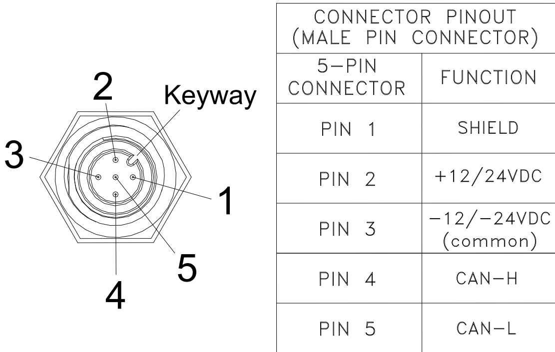
Figure 13: CAN Connector Pin Out details
